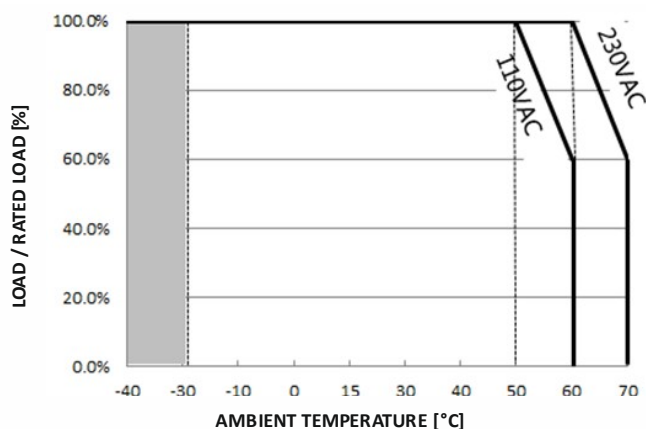
DERATING CURVE
