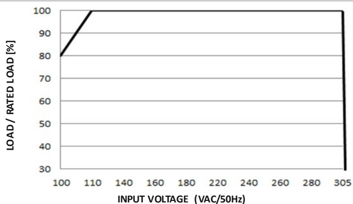
STATIC CHARACTERISTICS
