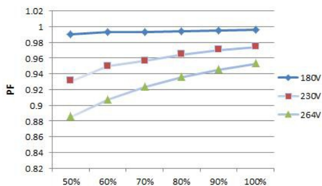
PF CURVE
