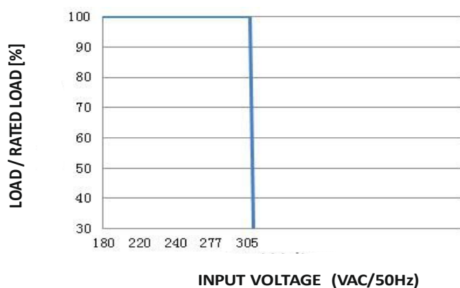
STATIC CHARACTERISTICS
