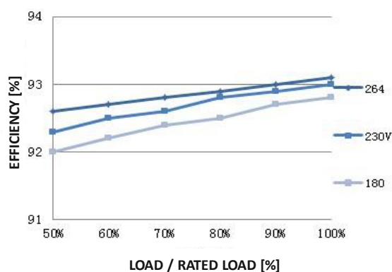
EFFICIENCY CURVE
