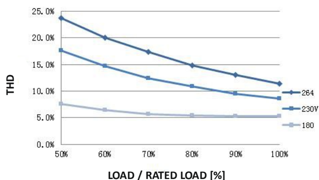
THD Curve
