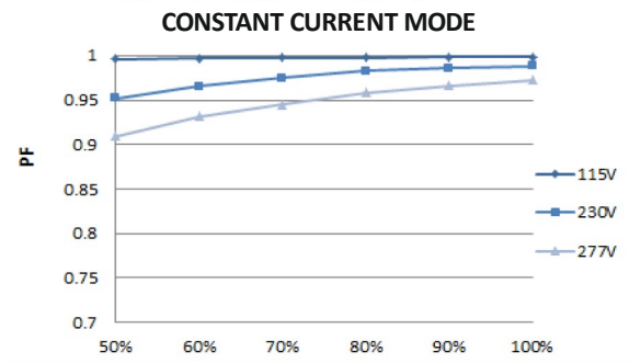
PF CURVE
