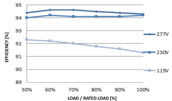
EFFICIENCY CURVE
