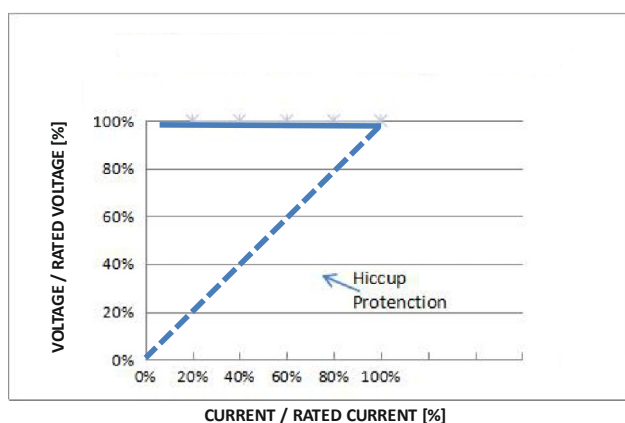
I-V CURVE
