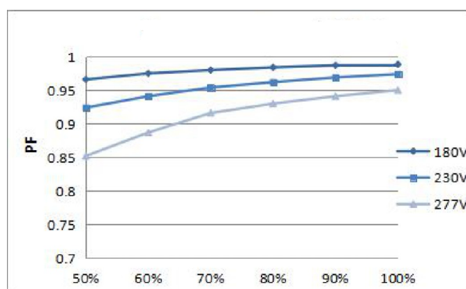
PF CURVE
