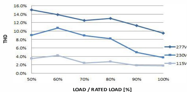
THD Curve
