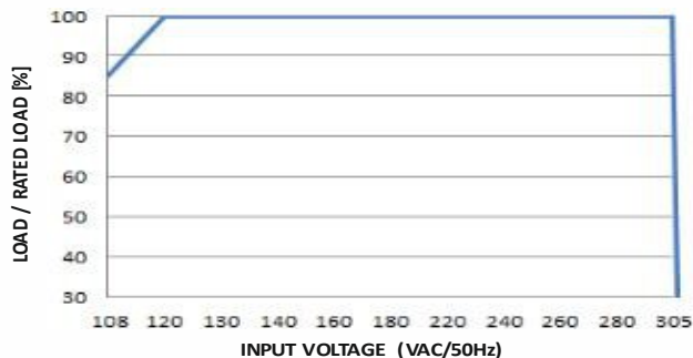
STATIC CHARACTERISTICS
