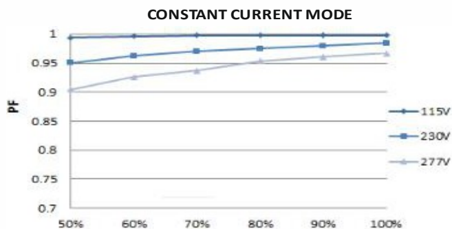
PF CURVE
