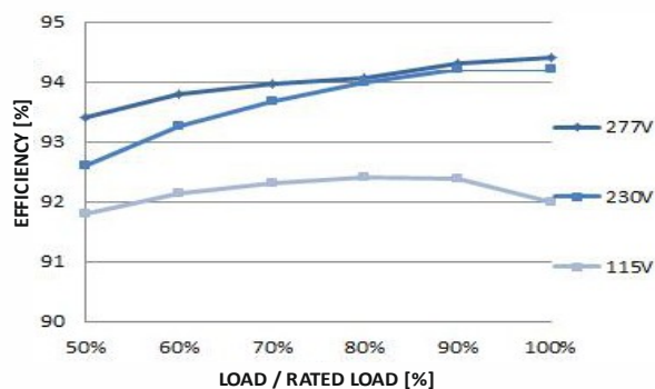
EFFICIENCY CURVE
